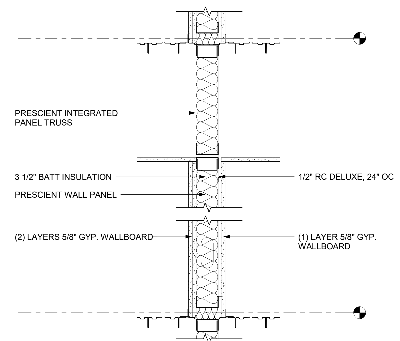
⑦ Demising/Corridor Prescient Wall - (TYP) 1 1/2" = 1'-0"
